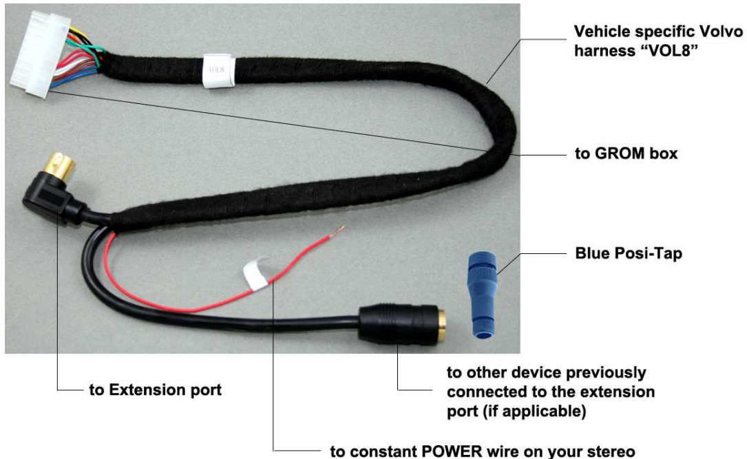
Picture 1: VOL8 vehicle specific harness and Posi-Tap
