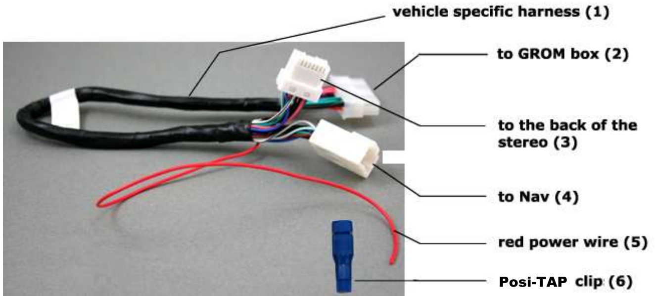
Picture 1: NIS2 vehicle specific harness
